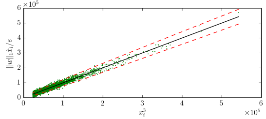
Figure 9: Plot of pairs (\|w\|_1 \hat{x}_i / s, x_i^3) on ML-S. The solid line is the reference for equality. Two dashed lines are for x_i^3 \pm \delta x_i^3 .
