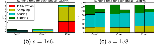
Figure 6: Performance of using prefiltering. The left bars in (b) and (c) are for t' = s and the right are for t' = s/10 .
