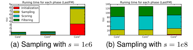
Figure 5: Running time in details for LastFM.
